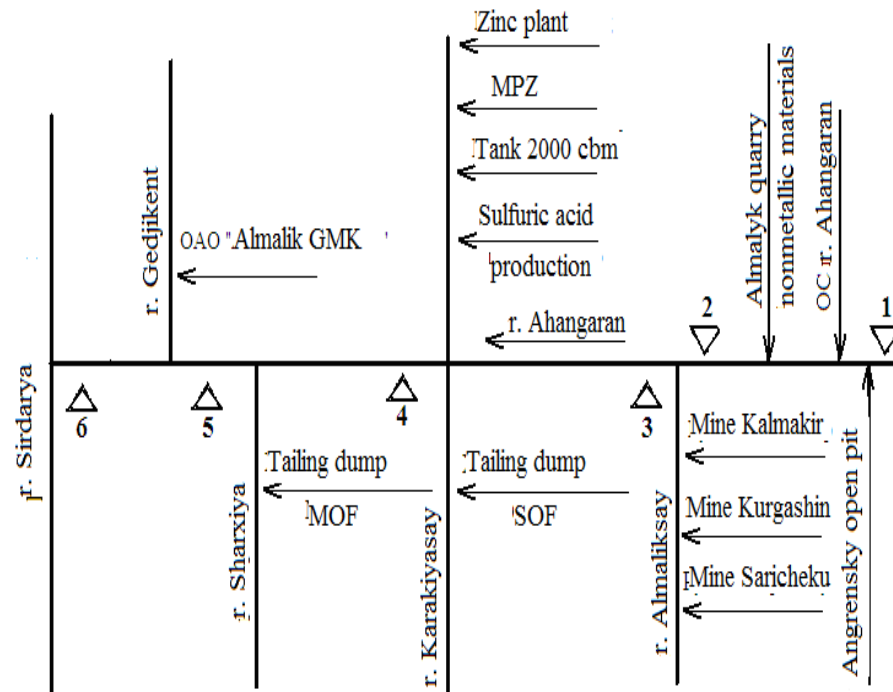
Fig. 2. Linear layout of sections for monitoring pollution of the river Akhangaran
