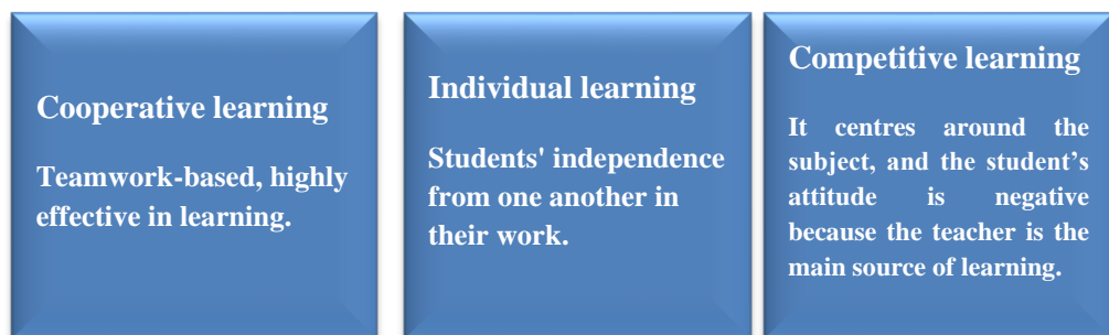
Fig. 3: Learning Types
