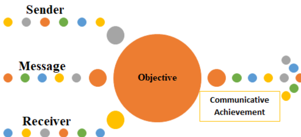
Fig. 2: Communication Elements
